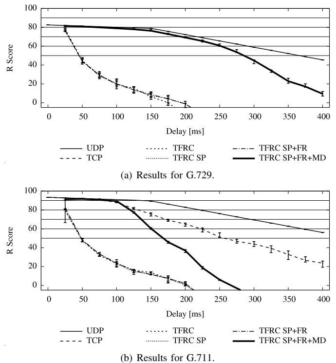
Fig. 5. Median R scores over 15 runs with corresponding interquartile gaps as error bars, for six different transport protocols and varying one-way delays from 0 to 400 ms and no losses, using G.729 and G.711.
